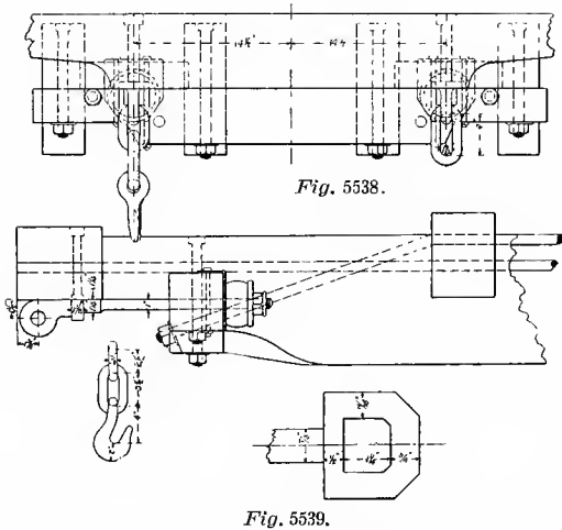
Fig. 5538. PLATFORM SAFETY-CHAINS FOR PASSENGER EQUIPMENT. Recommended Practice, adopted in 1893.
